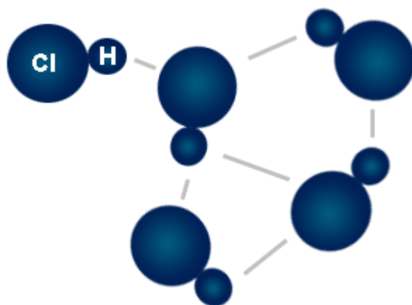
Figure 2-2: Dipole-dipole forces among HCl molecules
